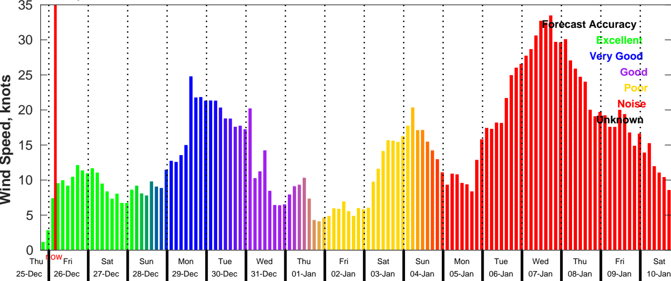
GFS Wind Speed Forecast for NDBC 42040 from 25-Dec-2025 19:00:00 to 10-Jan-2026 19:00:00
