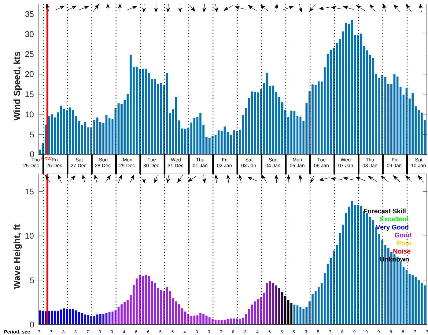
Wind & Wave Forecast for NDBC 42040 from 25-Dec-2025 19:00:00 to 10-Jan-2026 19:00:00
