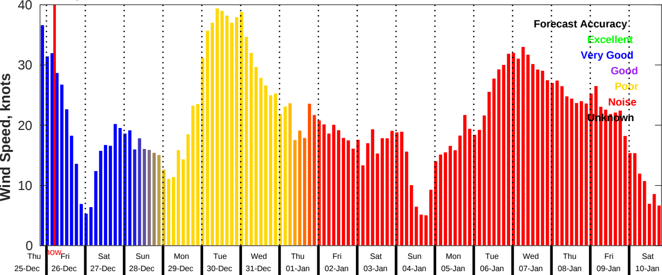
GFS Wind Speed Forecast for NDBC 44008 from 25-Dec-2025 20:00:00 to 10-Jan-2026 20:00:00
