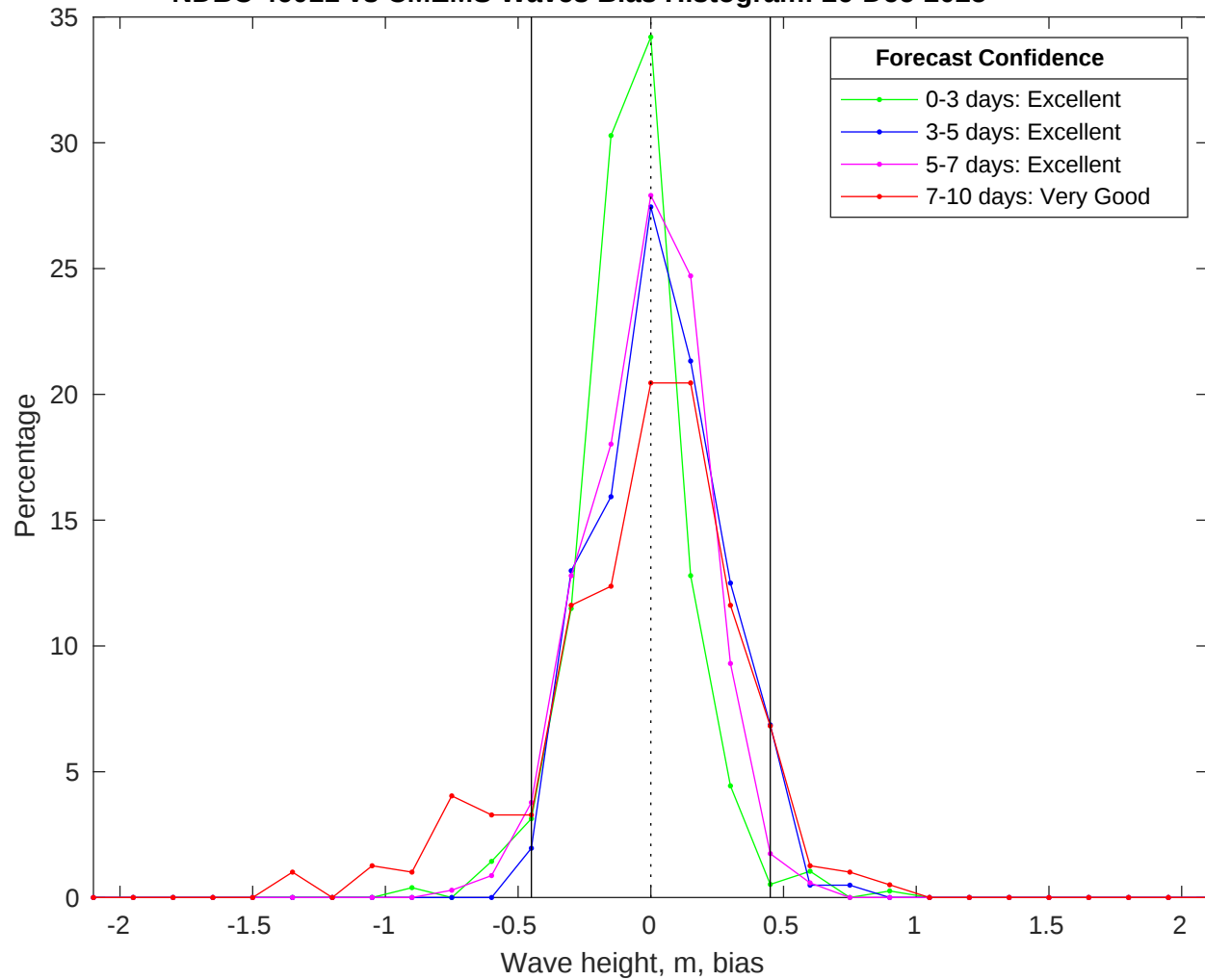
NDBC 46011 vs CMEMS Waves Bias Histogram: 26-Dec-2025
