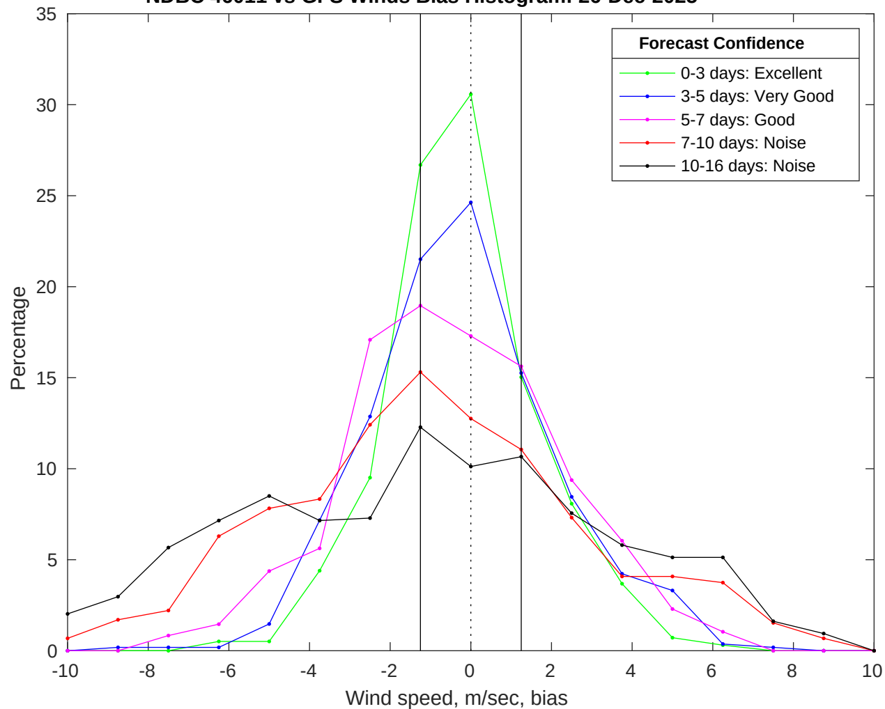
NDBC 46011 vs GFS Winds Bias Histogram: 26-Dec-2025
