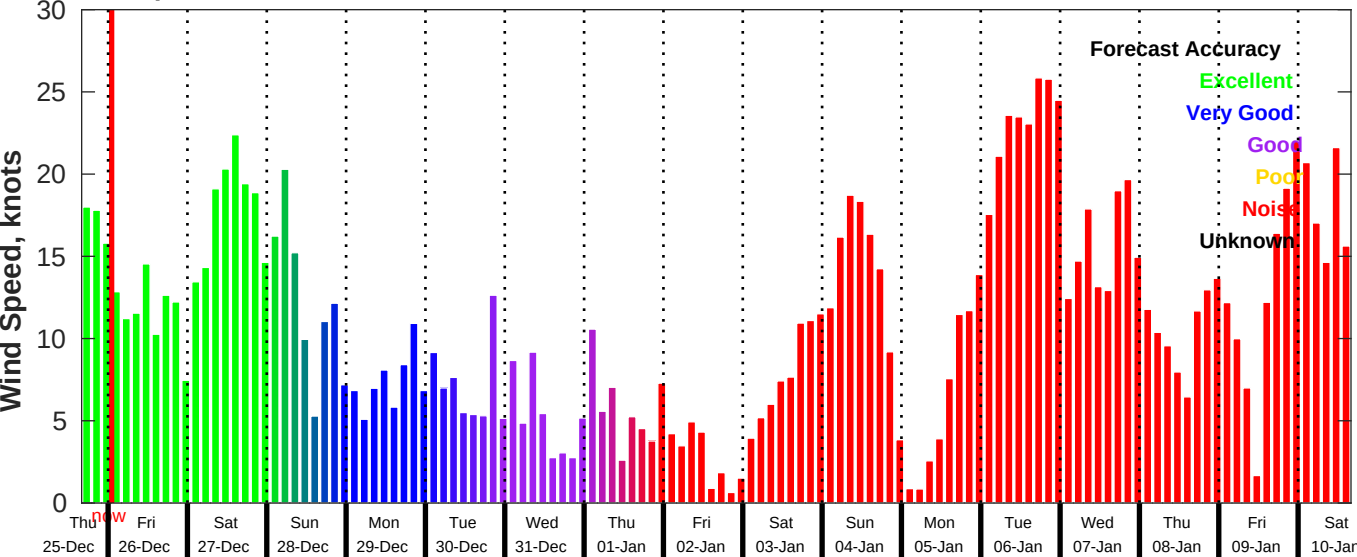
GFS Wind Speed Forecast for NDBC 46011 from 25-Dec-2025 16:00:00 to 10-Jan-2026 16:00:00
