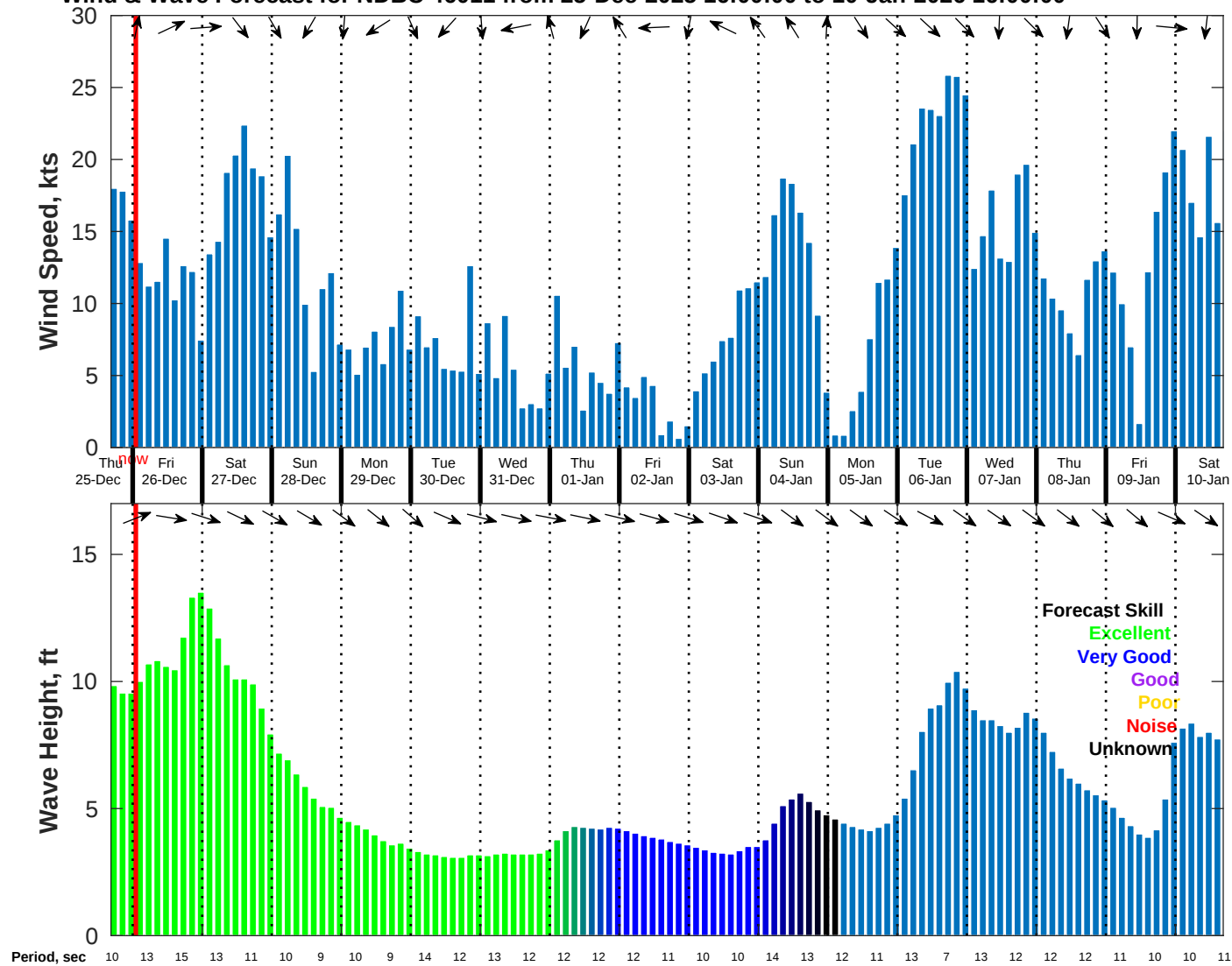
Wind & Wave Forecast for NDBC 46011 from 25-Dec-2025 16:00:00 to 10-Jan-2026 16:00:00
