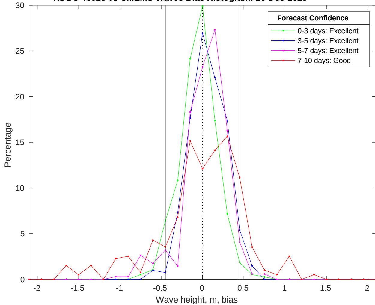
NDBC 46028 vs CMEMS Waves Bias Histogram: 26-Dec-2025
