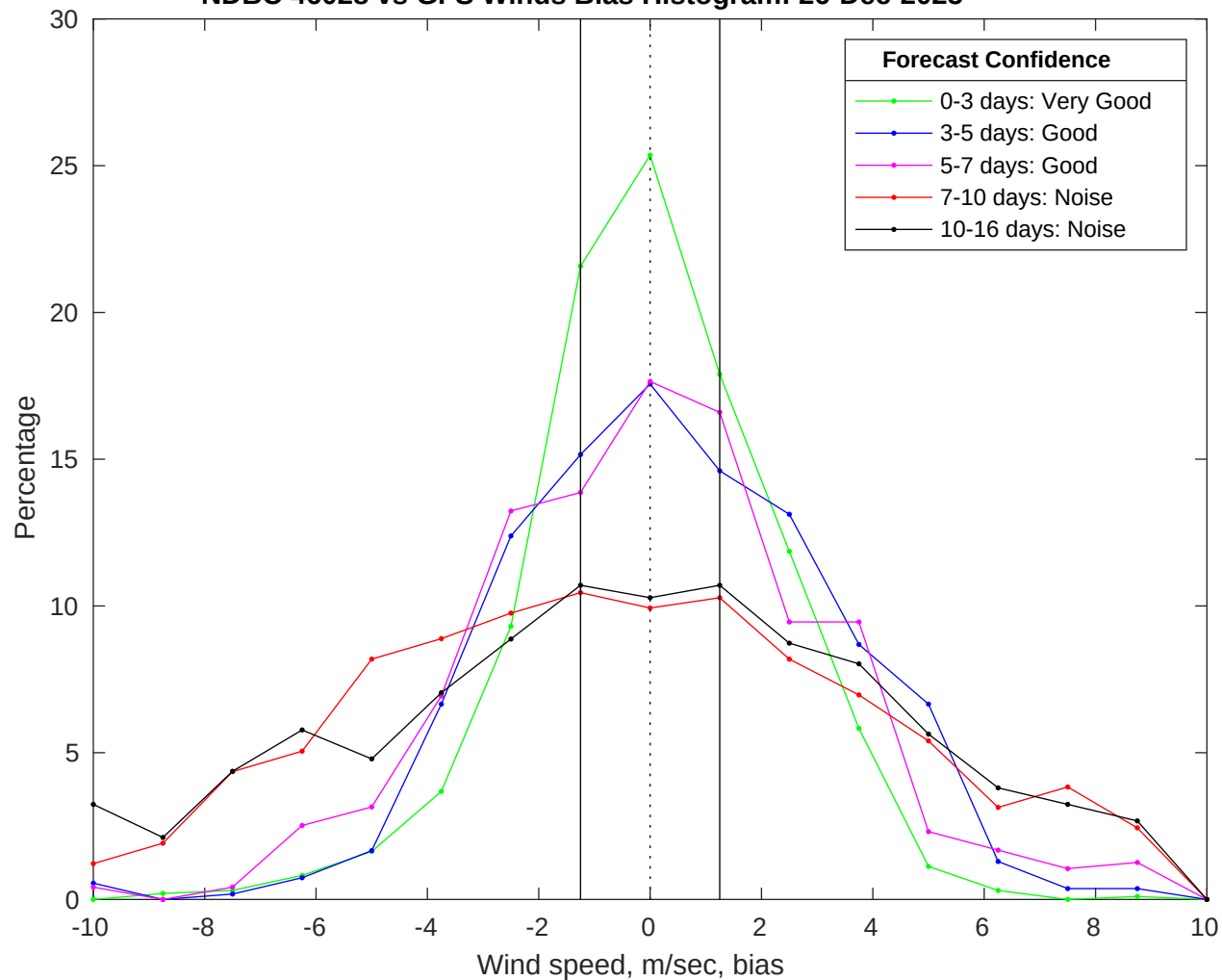
NDBC 46028 vs GFS Winds Bias Histogram: 26-Dec-2025
