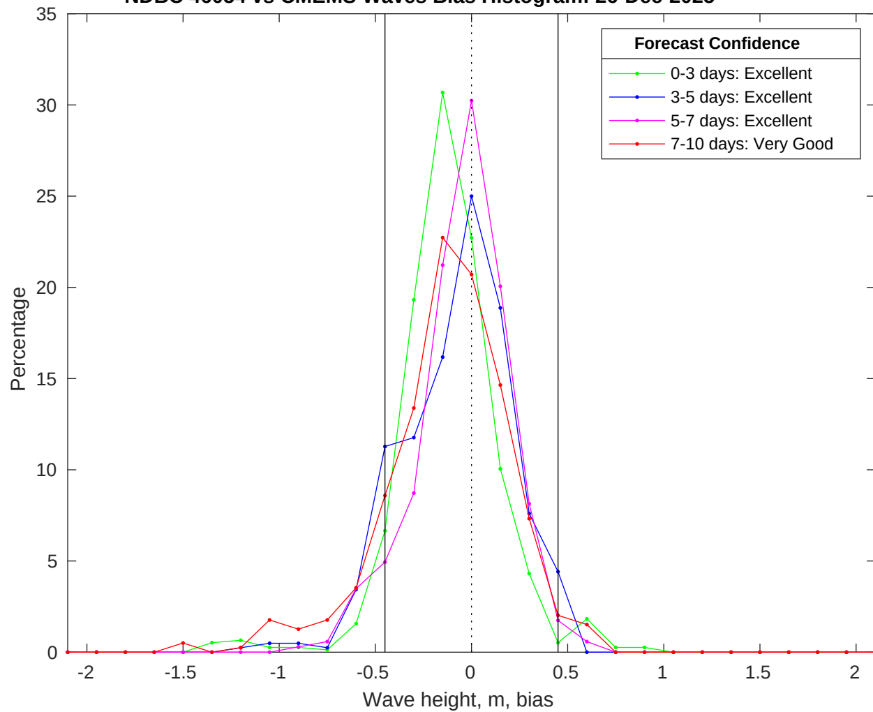
NDBC 46054 vs CMEMS Waves Bias Histogram: 26-Dec-2025
