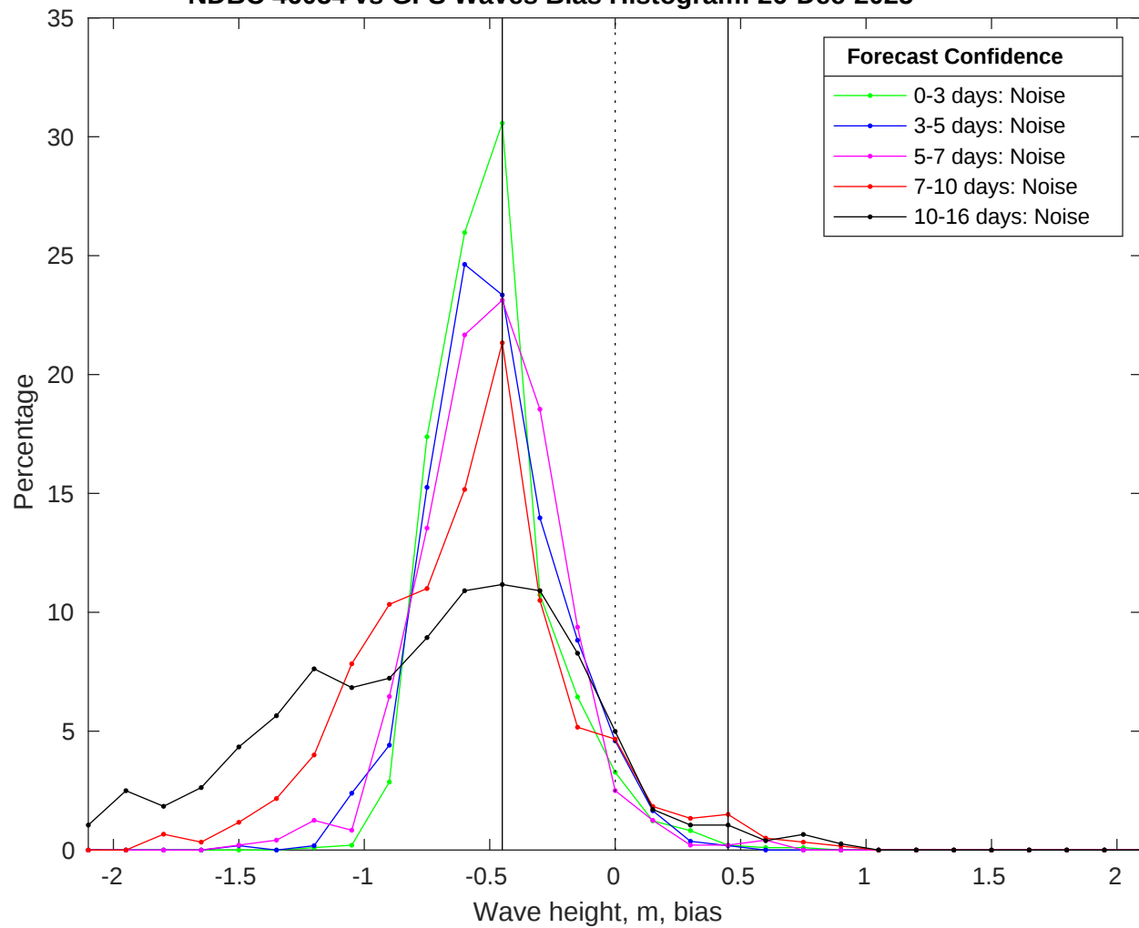
NDBC 46054 vs GFS Waves Bias Histogram: 26-Dec-2025
