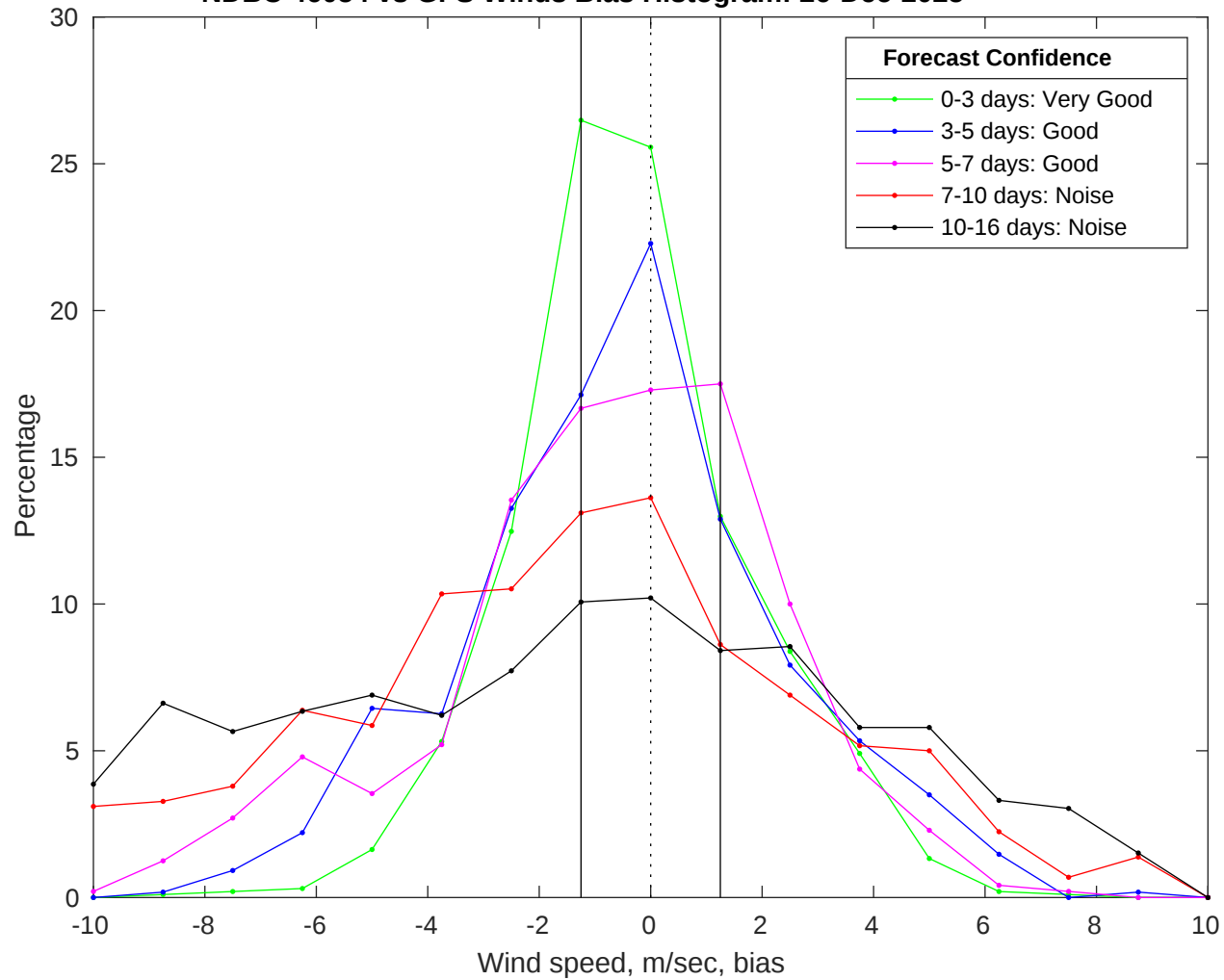
NDBC 46054 vs GFS Winds Bias Histogram: 26-Dec-2025
