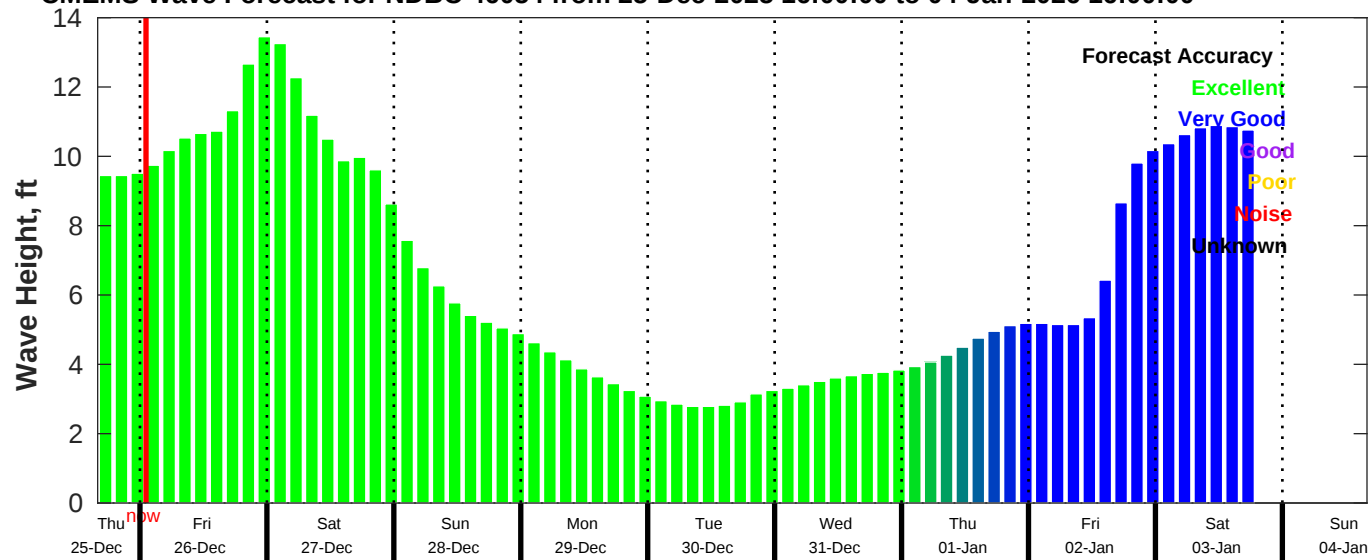
CMEMS Wave Forecast for NDBC 46054 from 25-Dec-2025 16:00:00 to 04-Jan-2026 16:00:00
