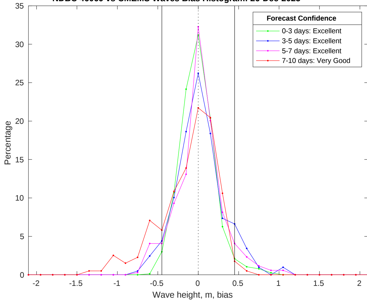
NDBC 46069 vs CMEMS Waves Bias Histogram: 26-Dec-2025
