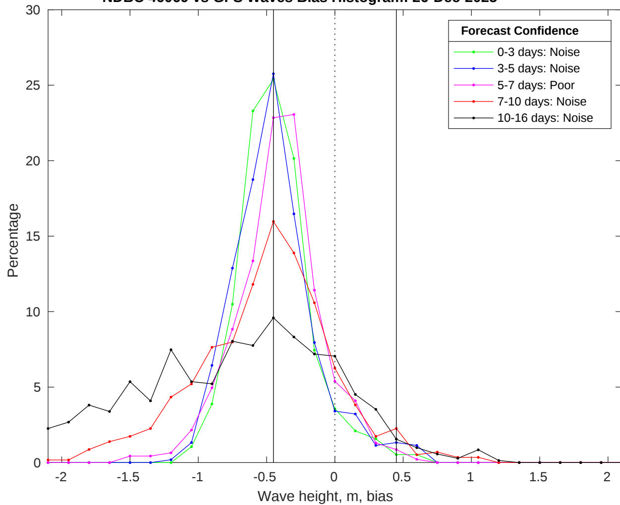
NDBC 46069 vs GFS Waves Bias Histogram: 26-Dec-2025
