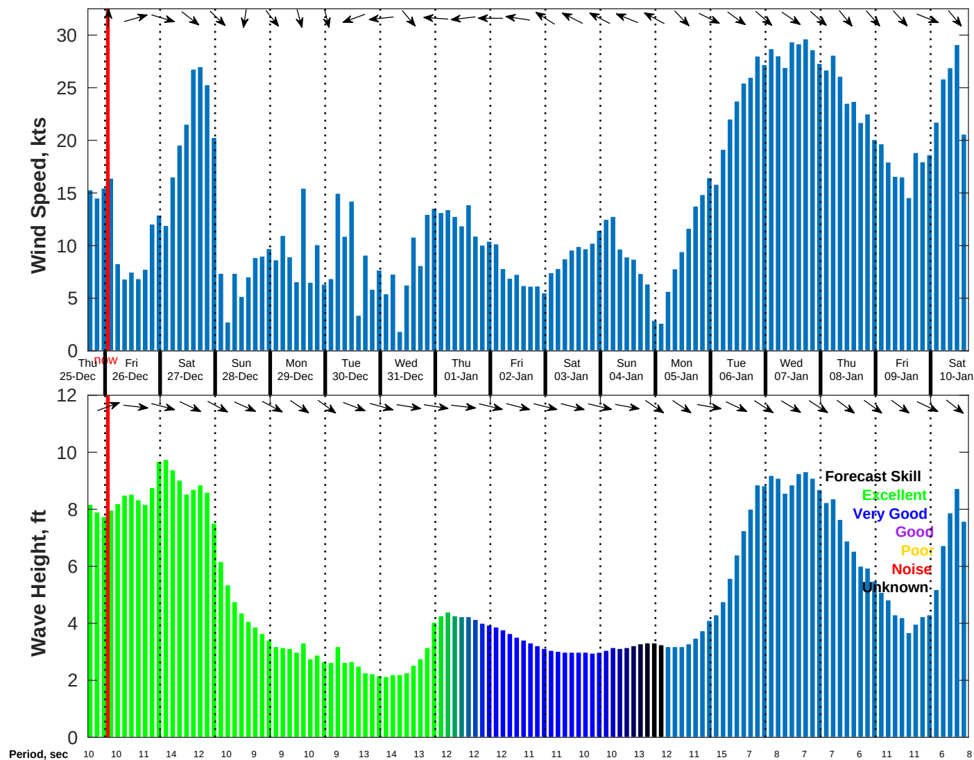
Wind & Wave Forecast for NDBC 46069 from 25-Dec-2025 16:00:00 to 10-Jan-2026 16:00:00
