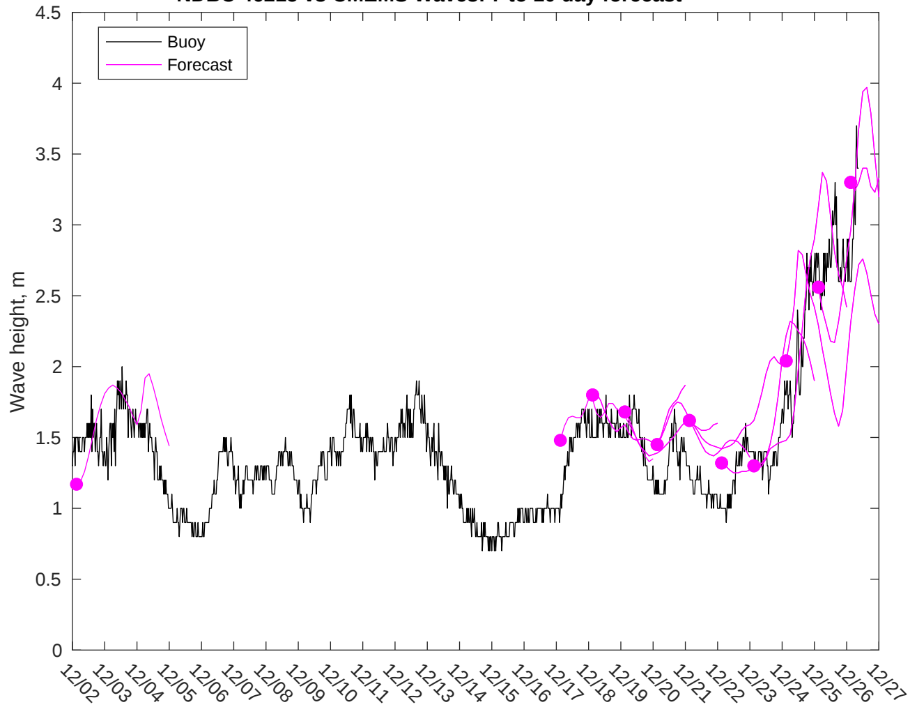
NDBC 46215 vs CMEMS Waves: 7 to 10 day forecast
