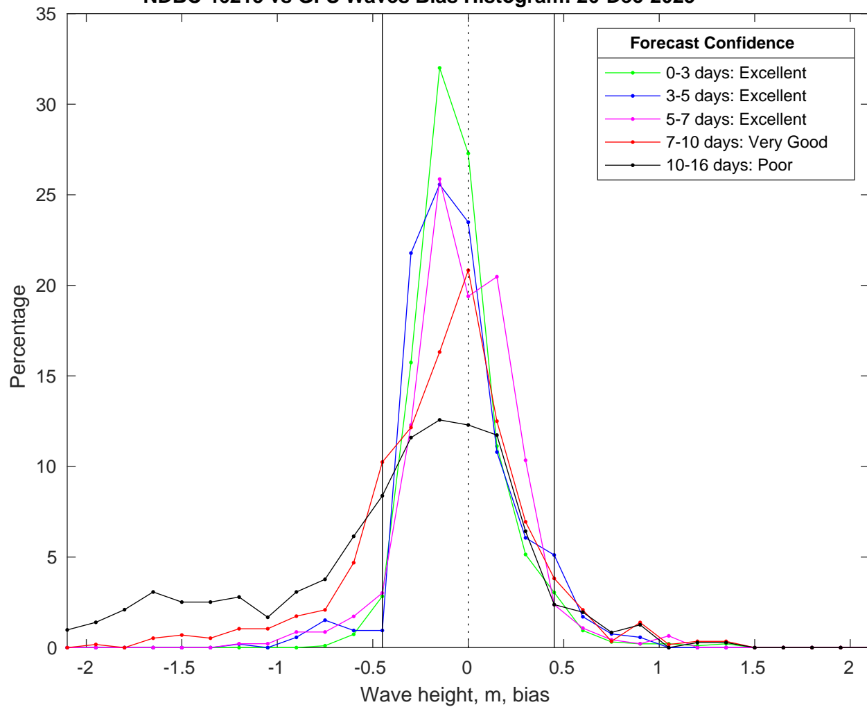
NDBC 46215 vs GFS Waves Bias Histogram: 26-Dec-2025
