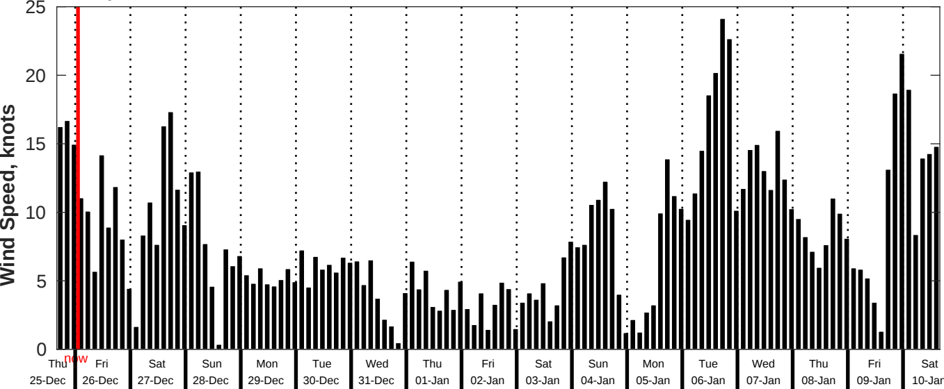
GFS Wind Speed Forecast for NDBC 46215 from 25-Dec-2025 16:00:00 to 10-Jan-2026 16:00:00
