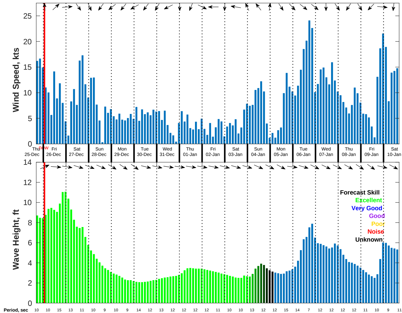
Wind & Wave Forecast for NDBC 46215 from 25-Dec-2025 16:00:00 to 10-Jan-2026 16:00:00
