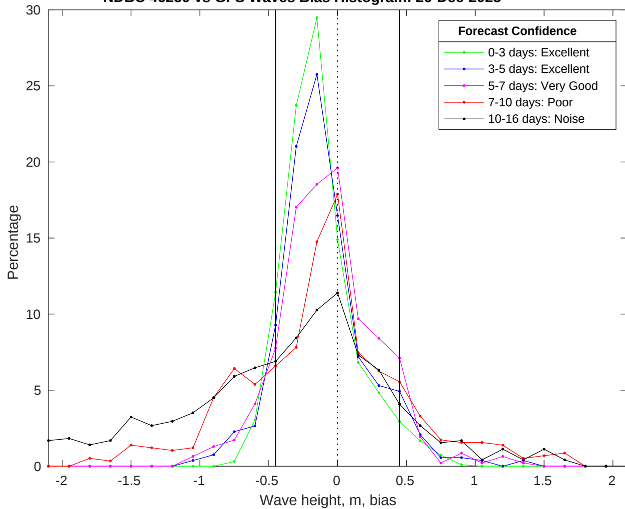
NDBC 46259 vs GFS Waves Bias Histogram: 26-Dec-2025
