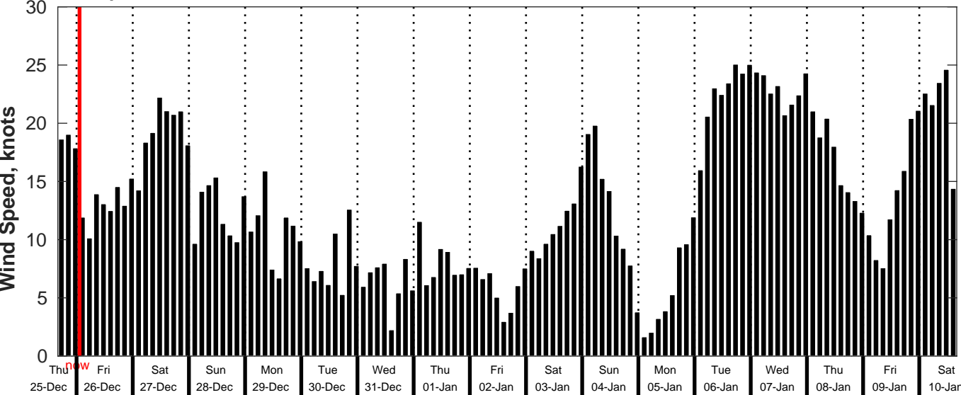
GFS Wind Speed Forecast for NDBC 46259 from 25-Dec-2025 16:00:00 to 10-Jan-2026 16:00:00
