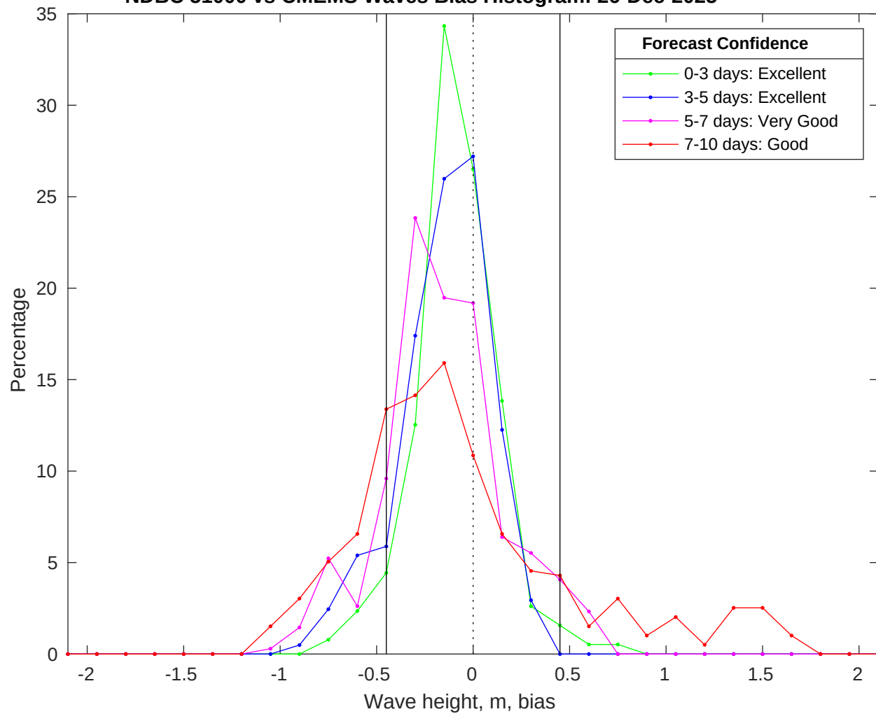
NDBC 51000 vs CMEMS Waves Bias Histogram: 26-Dec-2025
