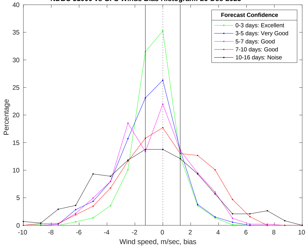
NDBC 51000 vs GFS Winds Bias Histogram: 26-Dec-2025
