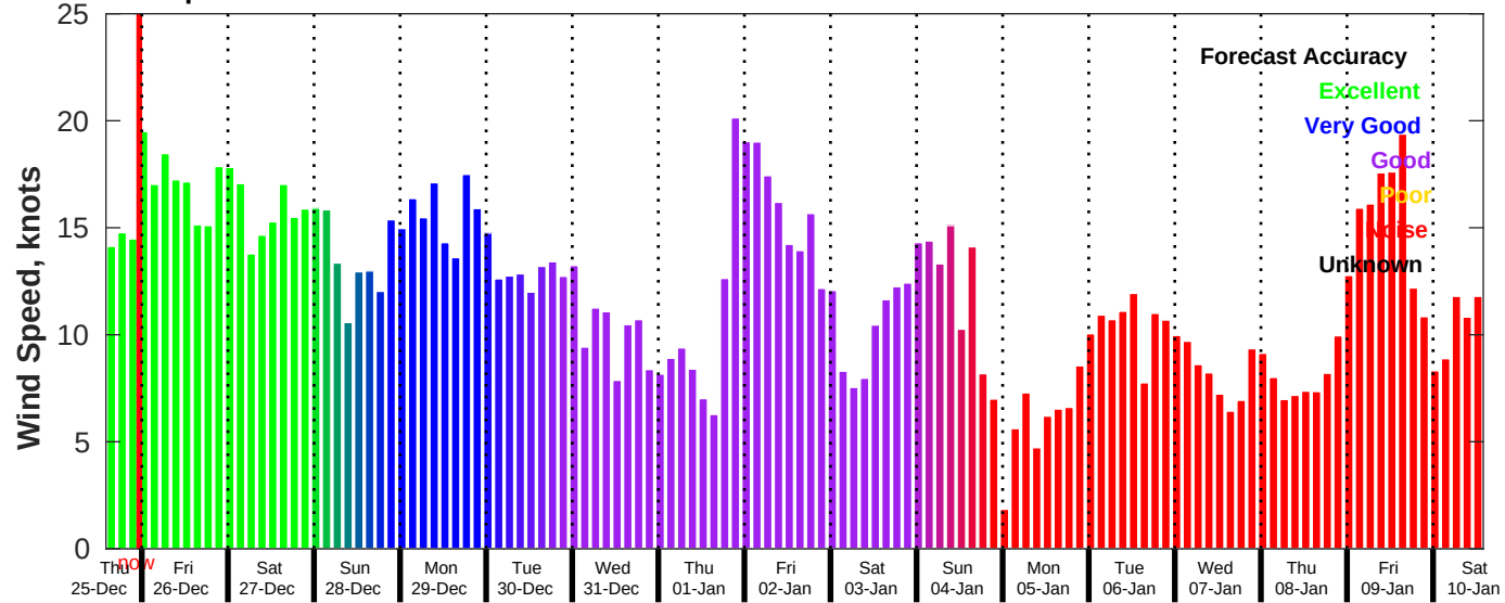
GFS Wind Speed Forecast for NDBC 51000 from 25-Dec-2025 14:00:00 to 10-Jan-2026 14:00:00
