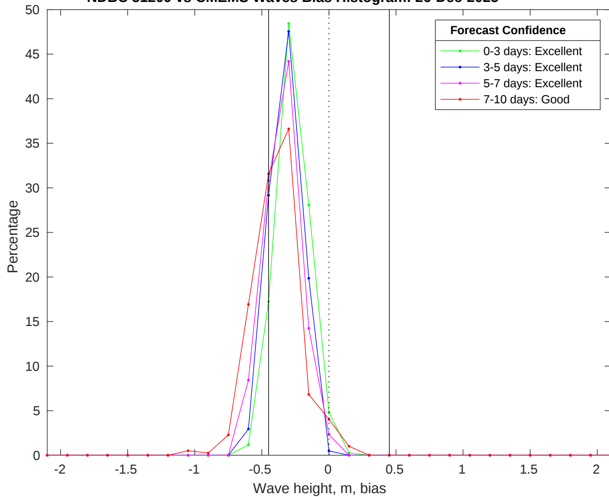
NDBC 51209 vs CMEMS Waves Bias Histogram: 26-Dec-2025
