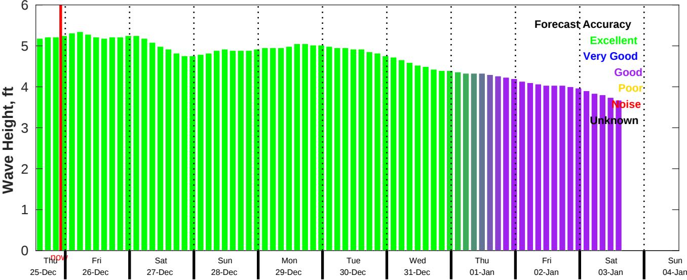
CMEMS Wave Forecast for NDBC 51209 from 25-Dec-2025 13:00:00 to 04-Jan-2026 13:00:00
