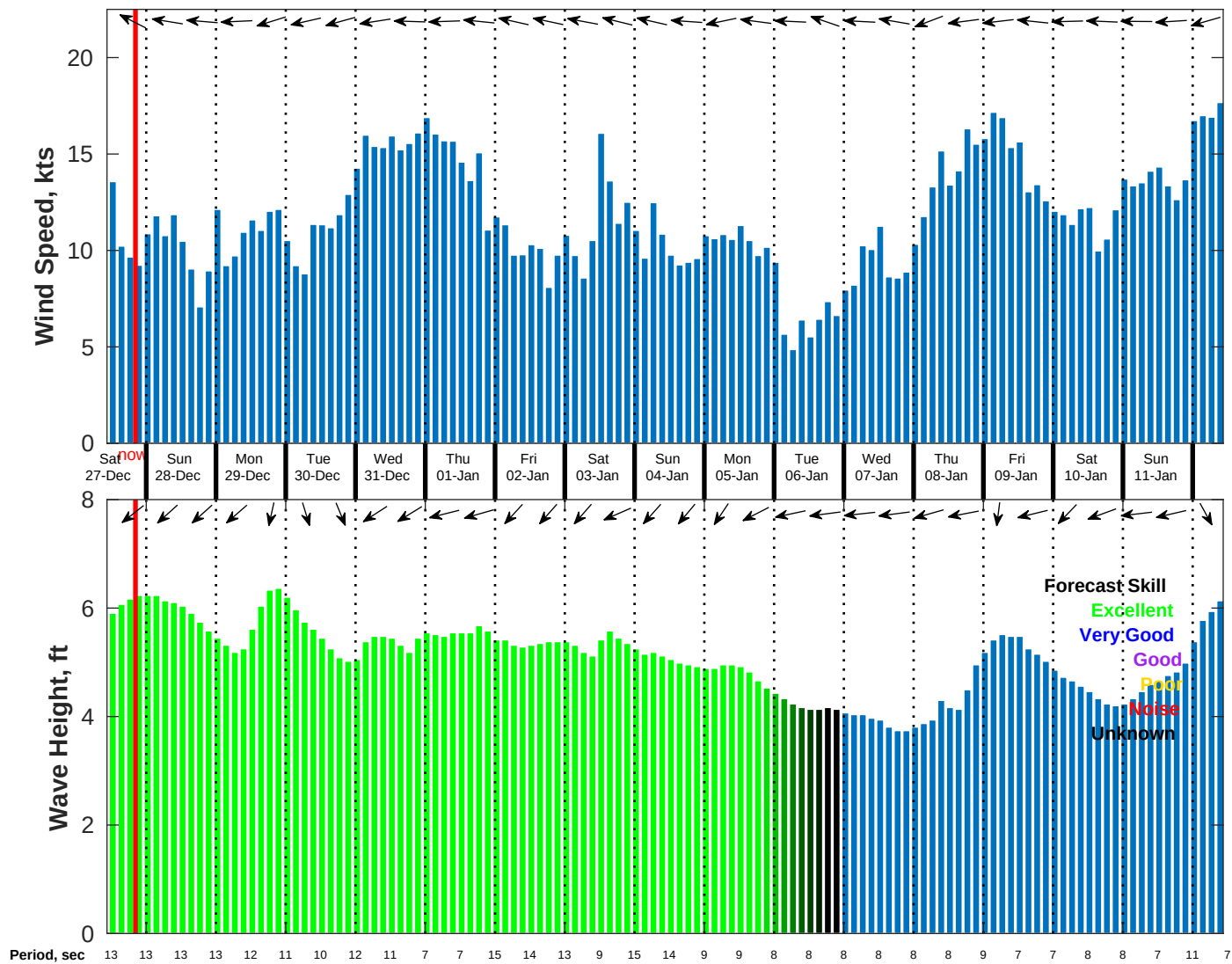
Wind & Wave Forecast for NDBC 52211 from 26-Dec-2025 11:00:00 to 11-Jan-2026 11:00:00
