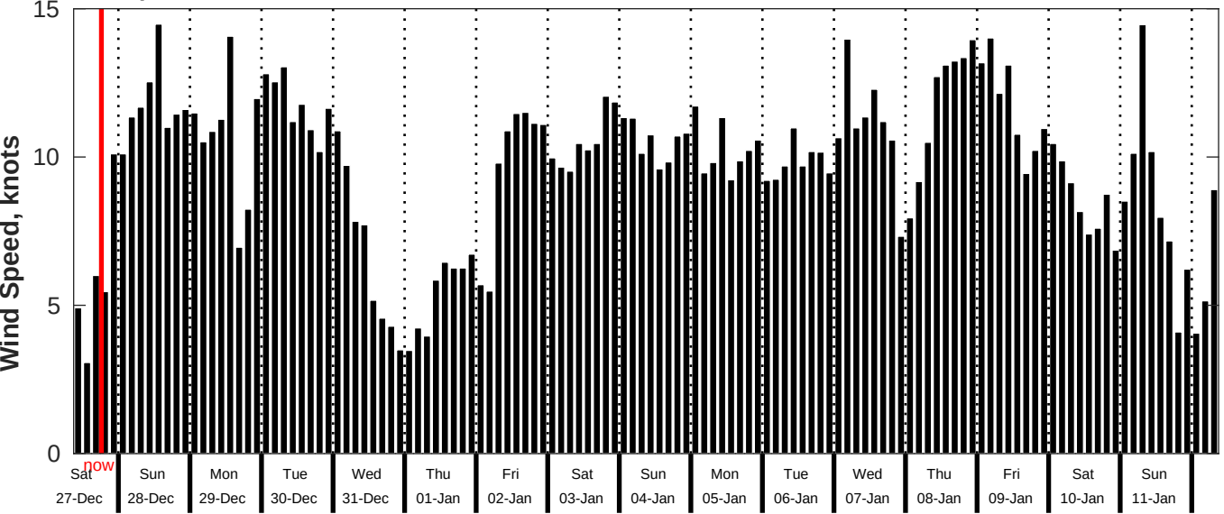
GFS Wind Speed Forecast for NDBC 52212 from 26-Dec-2025 09:00:00 to 11-Jan-2026 09:00:00
