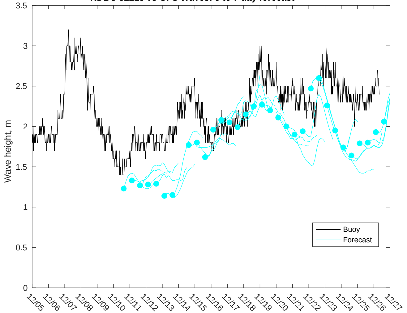
NDBC 52213 vs GFS Waves: 5 to 7 day forecast
