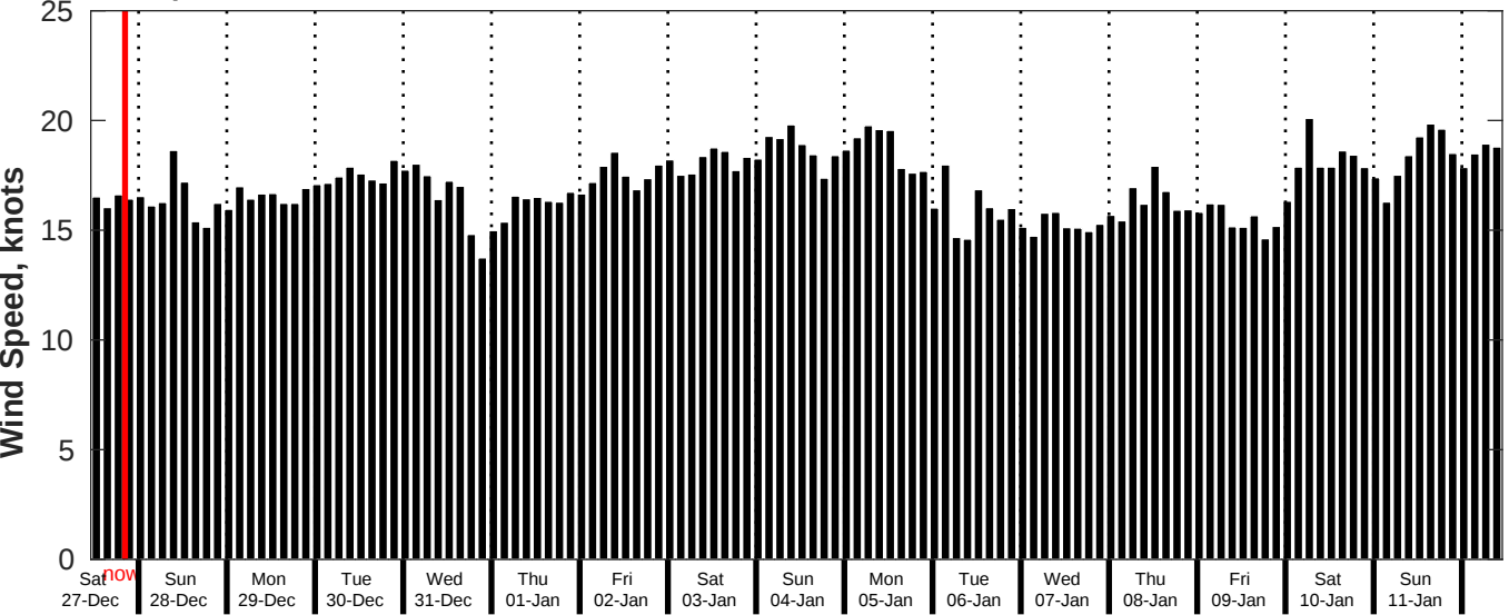
GFS Wind Speed Forecast for NDBC 52213 from 26-Dec-2025 11:00:00 to 11-Jan-2026 11:00:00
