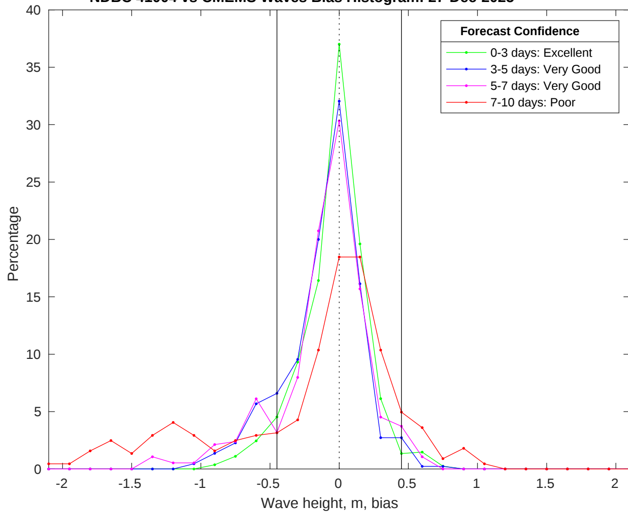
NDBC 41004 vs CMEMS Waves Bias Histogram: 27-Dec-2025
