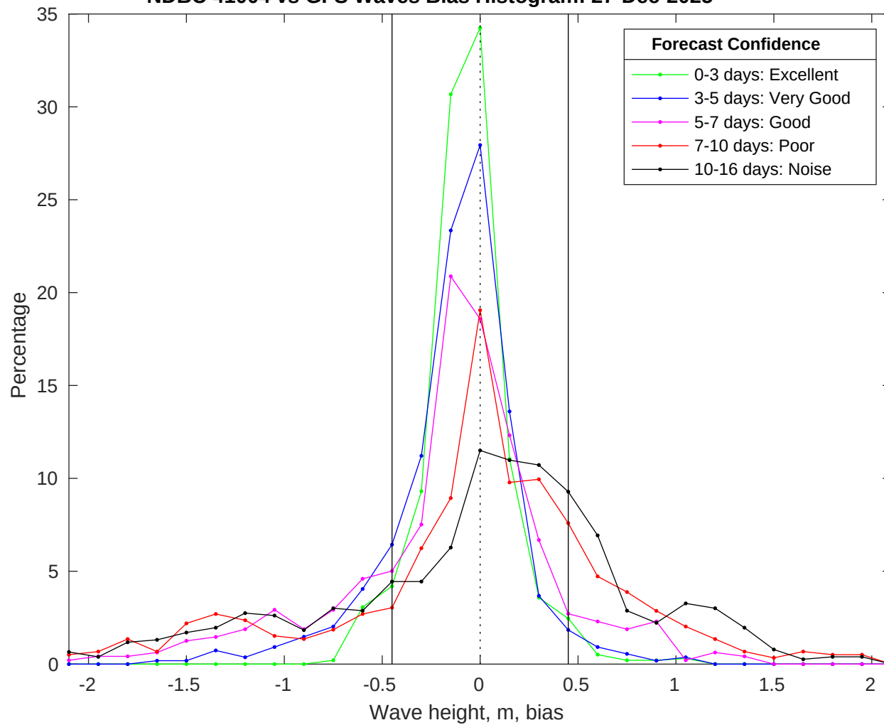
NDBC 41004 vs GFS Waves Bias Histogram: 27-Dec-2025
