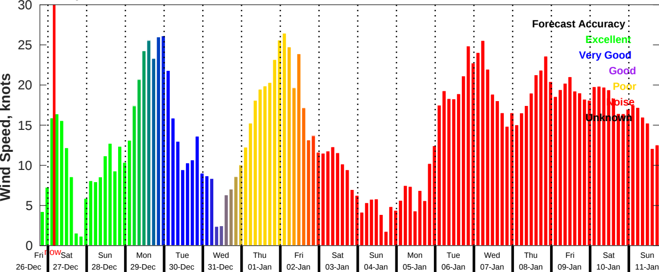
GFS Wind Speed Forecast for NDBC 41004 from 26-Dec-2025 19:00:00 to 11-Jan-2026 19:00:00
