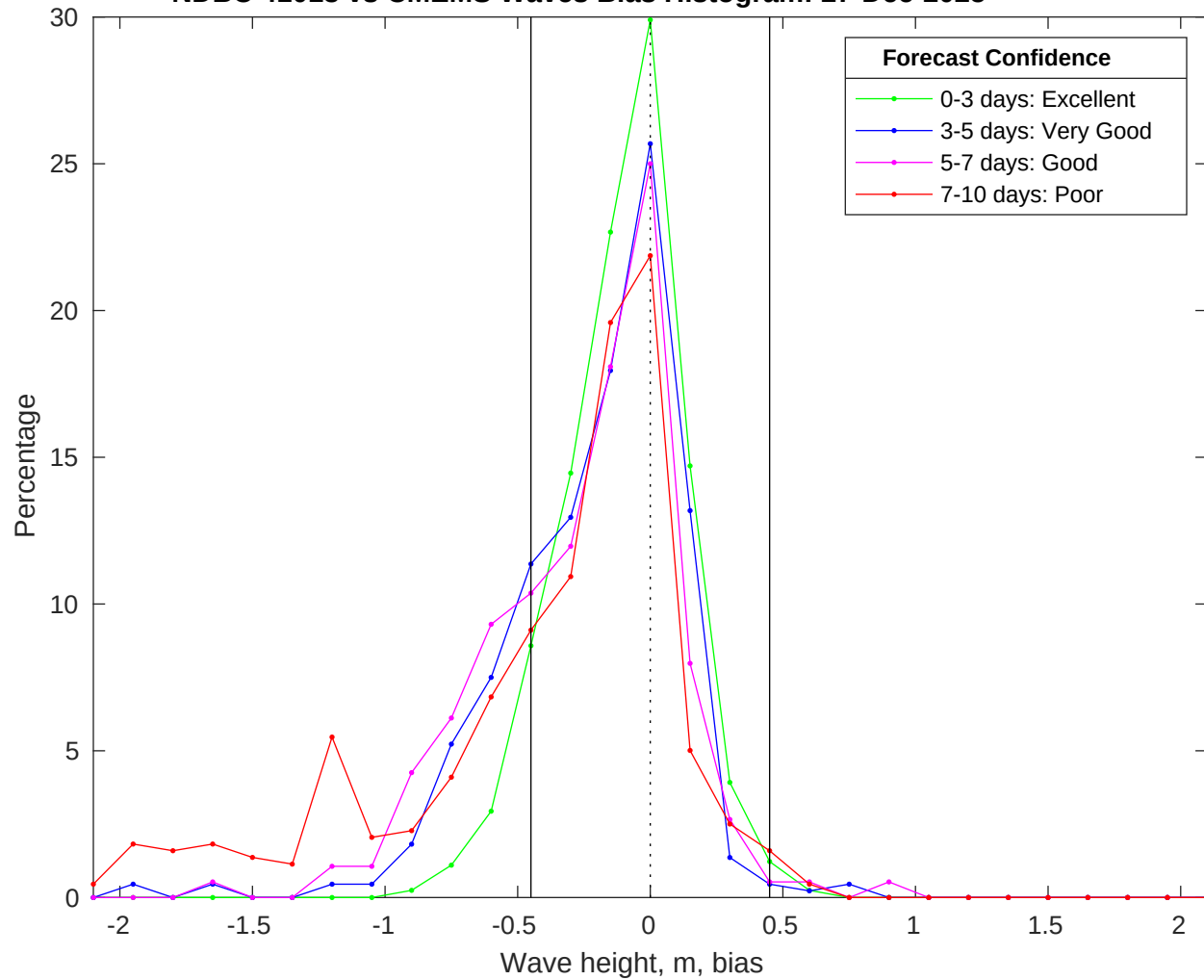
NDBC 41013 vs CMEMS Waves Bias Histogram: 27-Dec-2025
