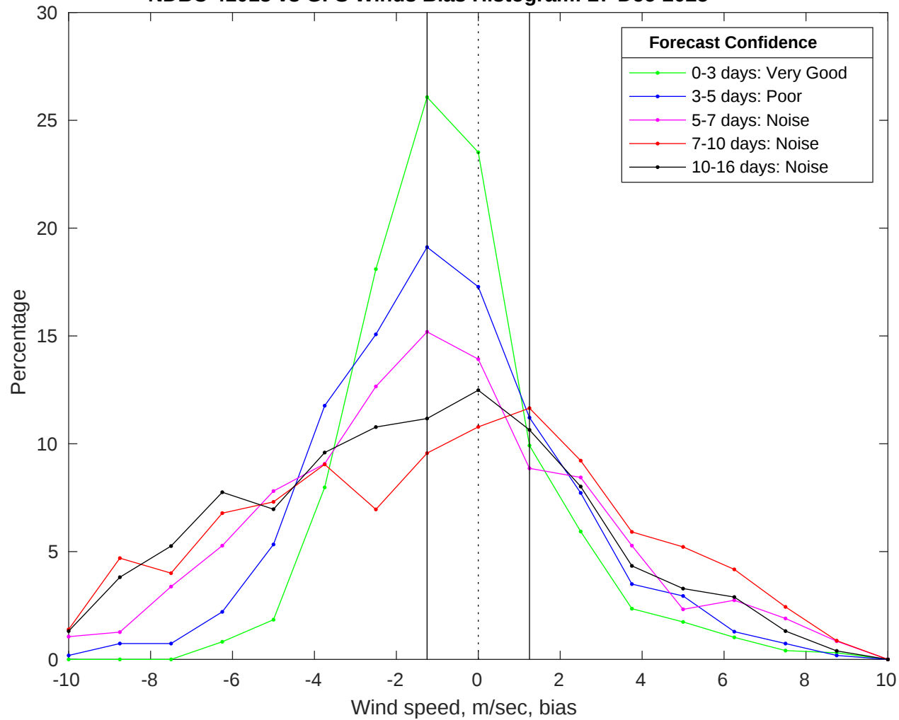
NDBC 41013 vs GFS Winds Bias Histogram: 27-Dec-2025
