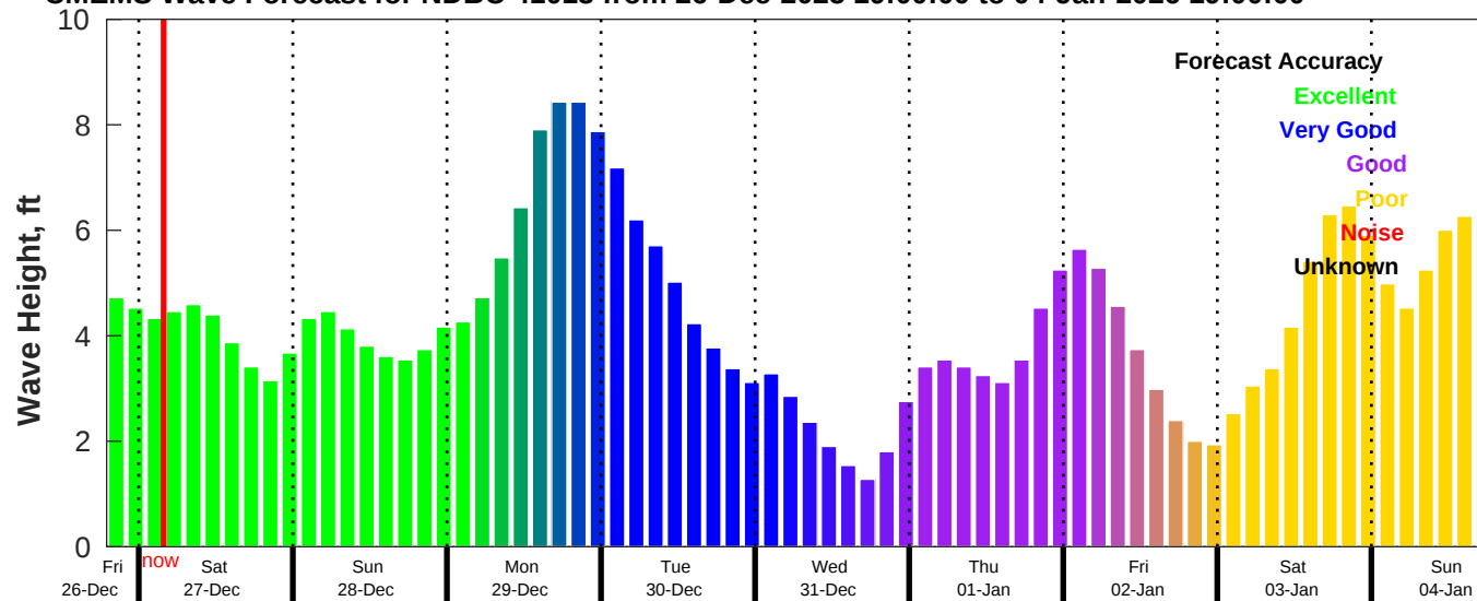
CMEMS Wave Forecast for NDBC 41013 from 26-Dec-2025 19:00:00 to 04-Jan-2026 19:00:00
