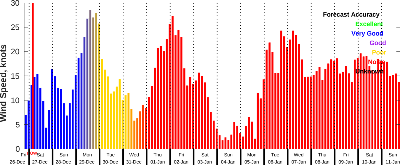
GFS Wind Speed Forecast for NDBC 41013 from 26-Dec-2025 19:00:00 to 11-Jan-2026 19:00:00
