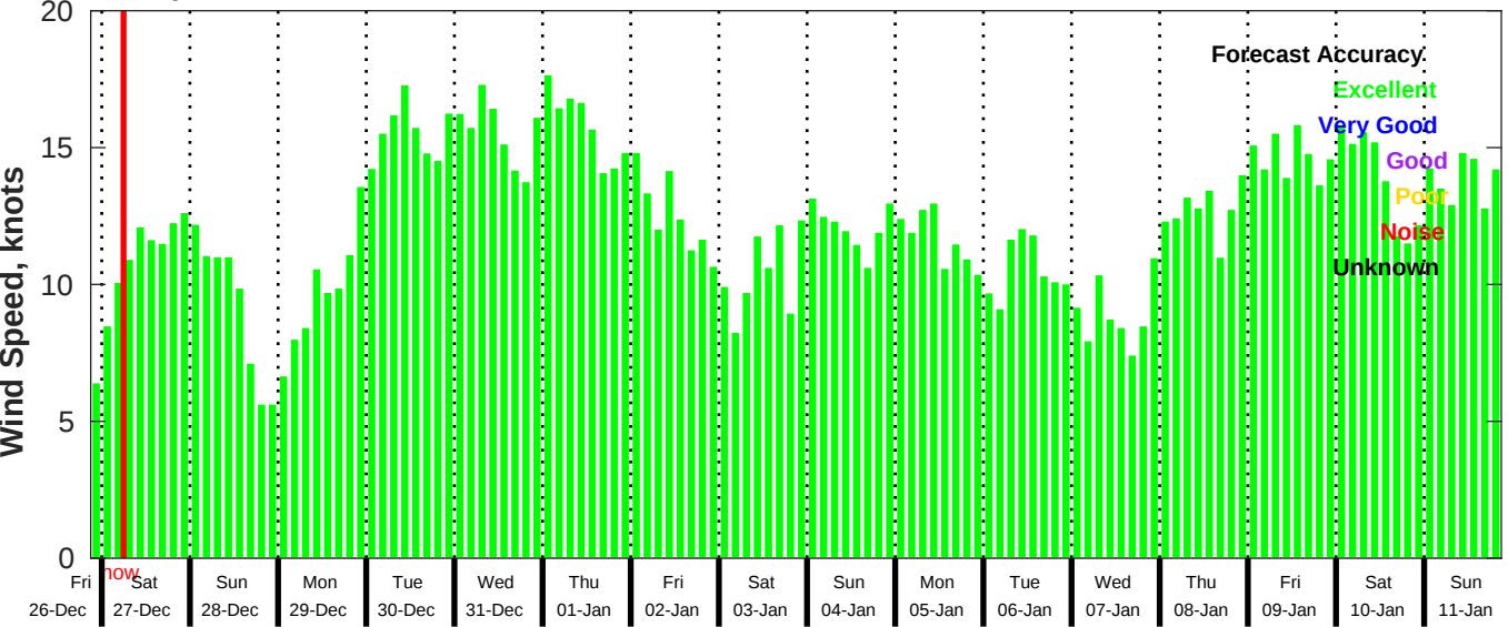
GFS Wind Speed Forecast for NDBC 41040 from 26-Dec-2025 21:00:00 to 11-Jan-2026 21:00:00
