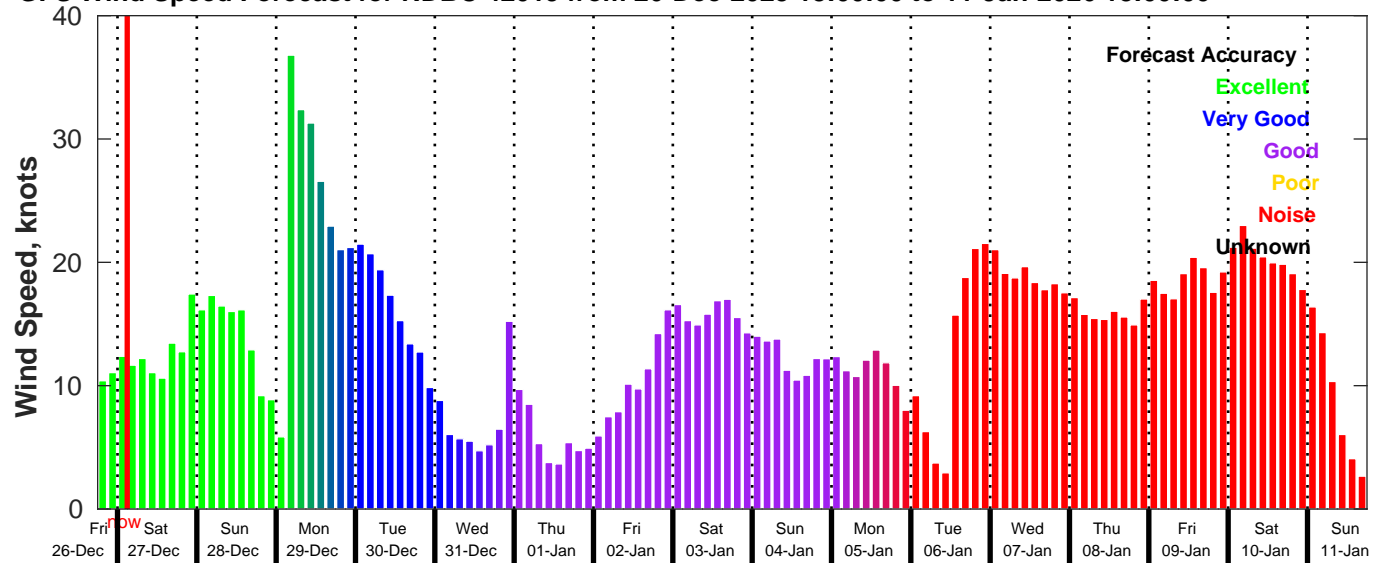
GFS Wind Speed Forecast for NDBC 42019 from 26-Dec-2025 18:00:00 to 11-Jan-2026 18:00:00
