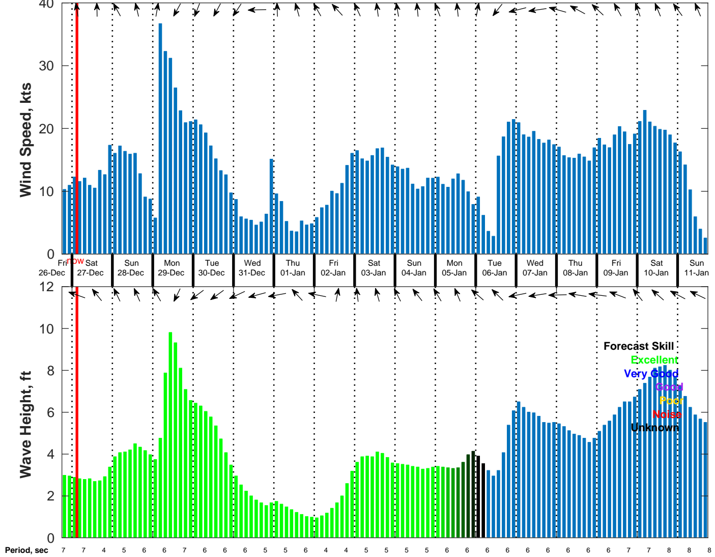
Wind & Wave Forecast for NDBC 42019 from 26-Dec-2025 18:00:00 to 11-Jan-2026 18:00:00
