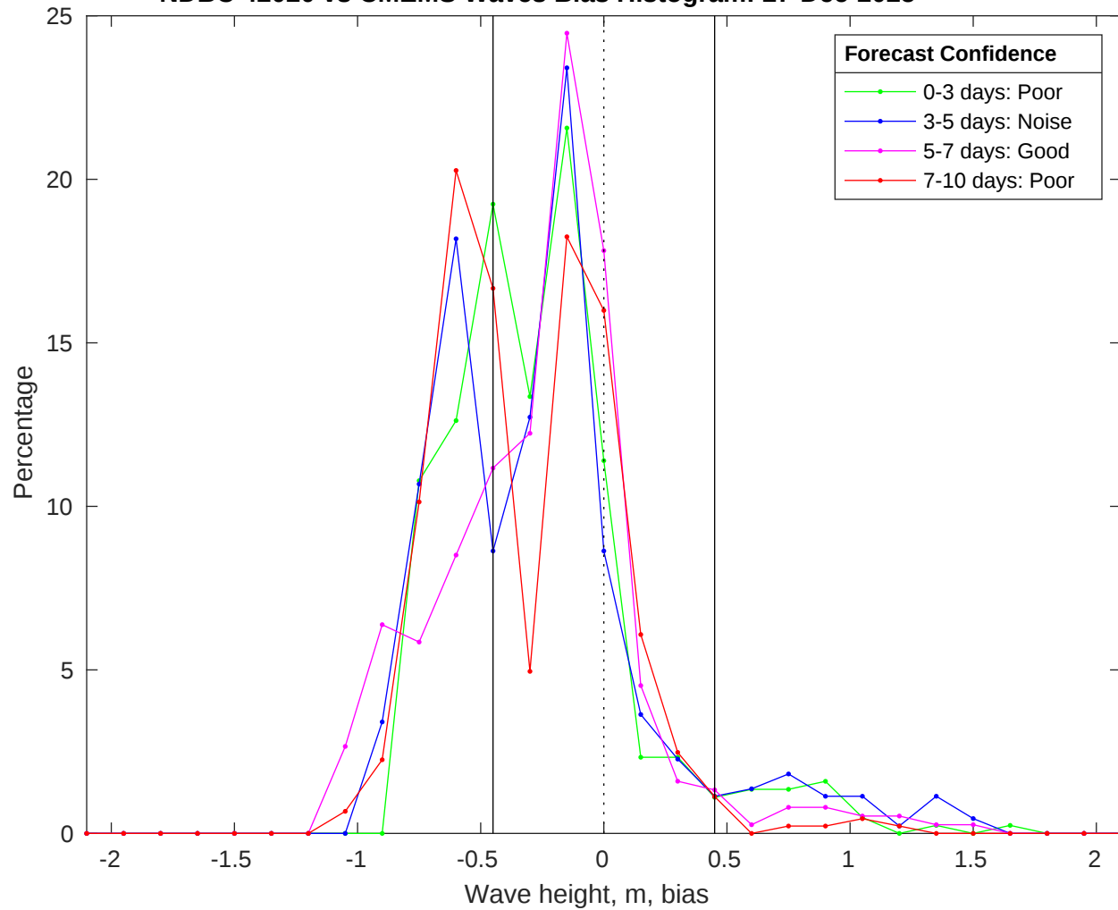
NDBC 42020 vs CMEMS Waves Bias Histogram: 27-Dec-2025
