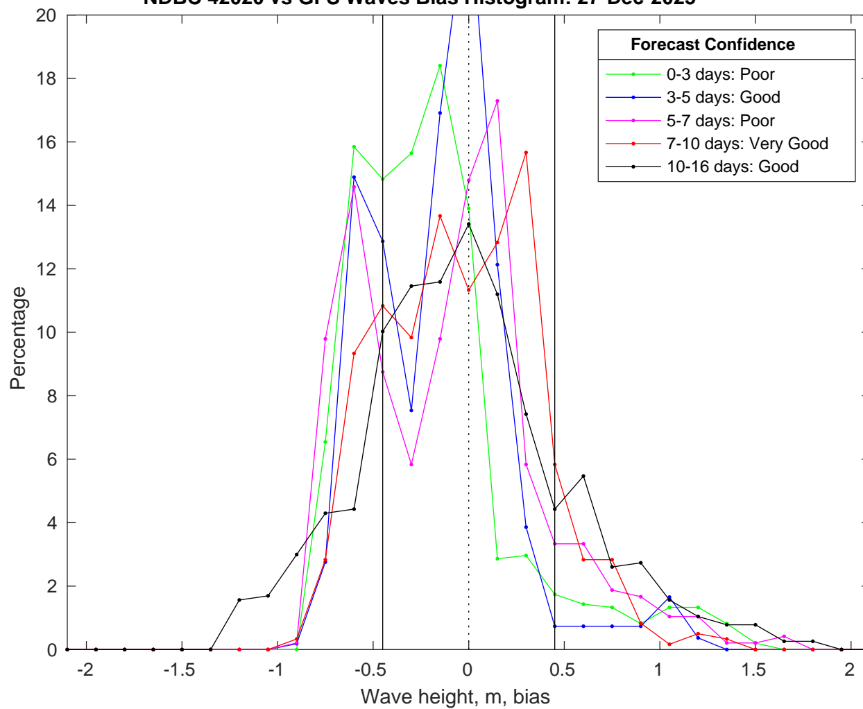
NDBC 42020 vs GFS Waves Bias Histogram: 27-Dec-2025
