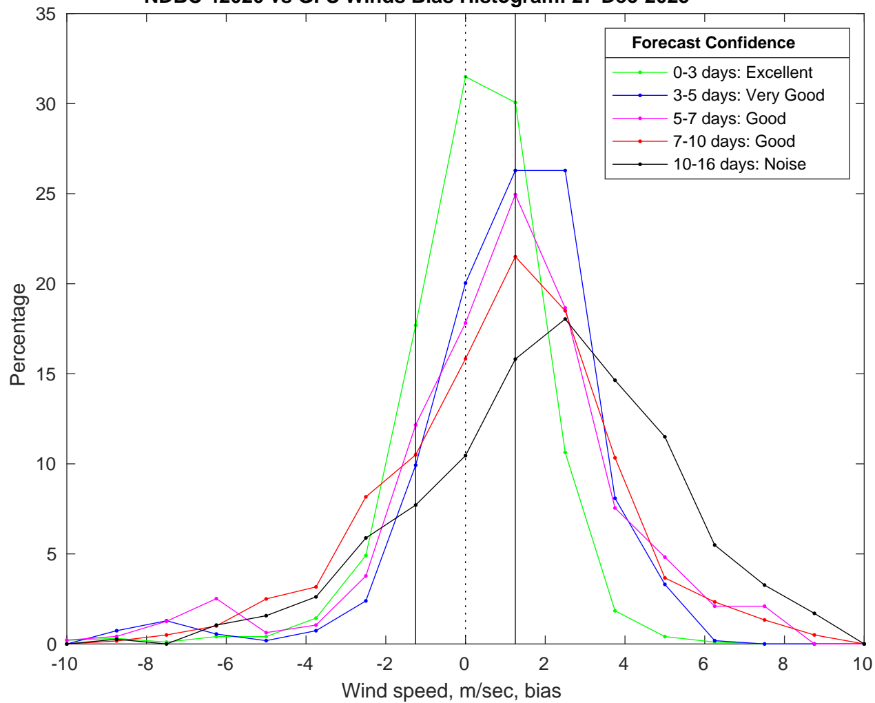
NDBC 42020 vs GFS Winds Bias Histogram: 27-Dec-2025
