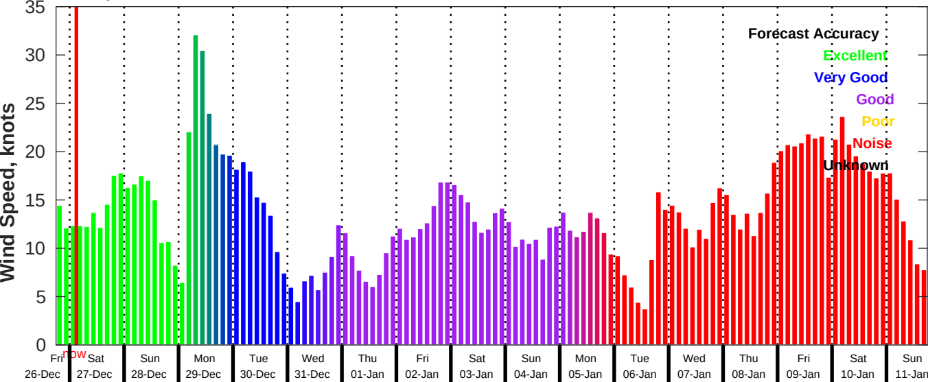
GFS Wind Speed Forecast for NDBC 42020 from 26-Dec-2025 18:00:00 to 11-Jan-2026 18:00:00
