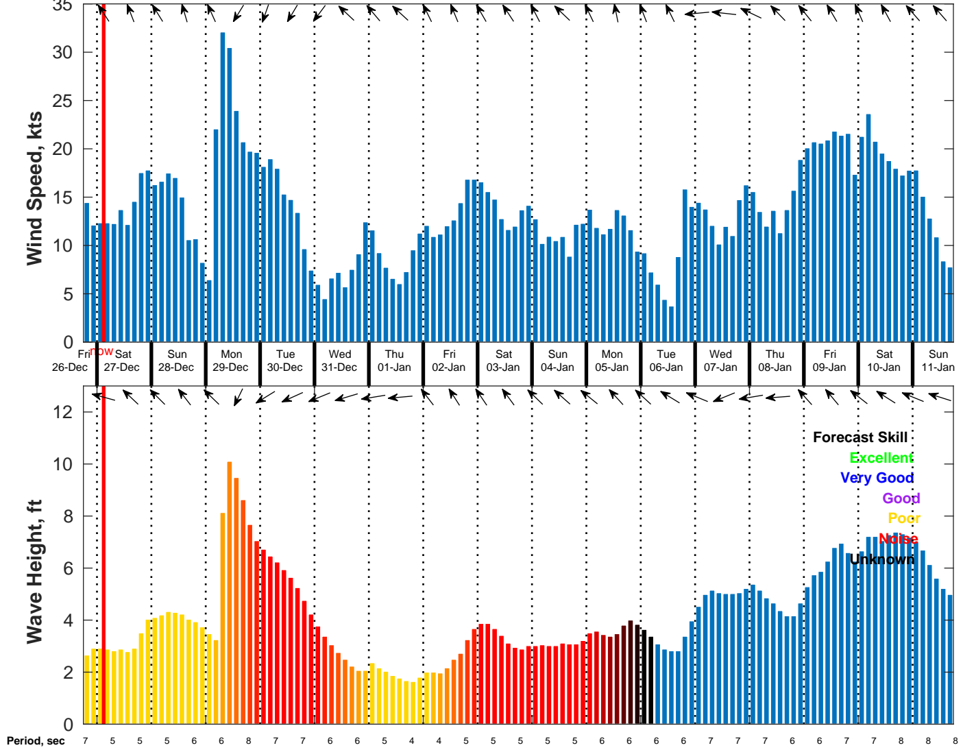
Wind & Wave Forecast for NDBC 42020 from 26-Dec-2025 18:00:00 to 11-Jan-2026 18:00:00
