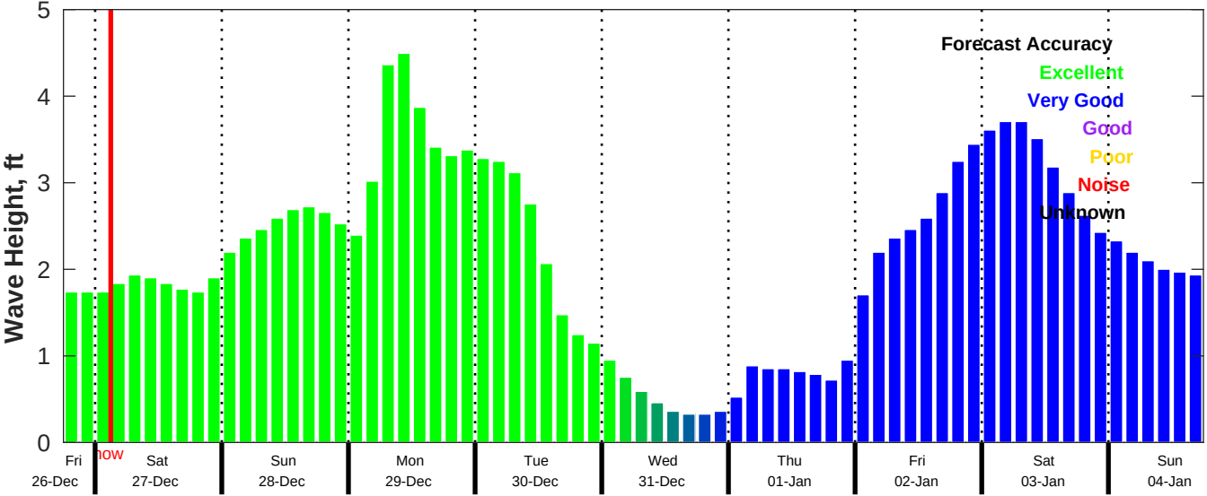
CMEMS Wave Forecast for NDBC 42035 from 26-Dec-2025 18:00:00 to 04-Jan-2026 18:00:00
