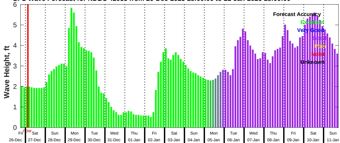
GFS Wave Forecast for NDBC 42035 from 26-Dec-2025 18:00:00 to 11-Jan-2026 18:00:00
