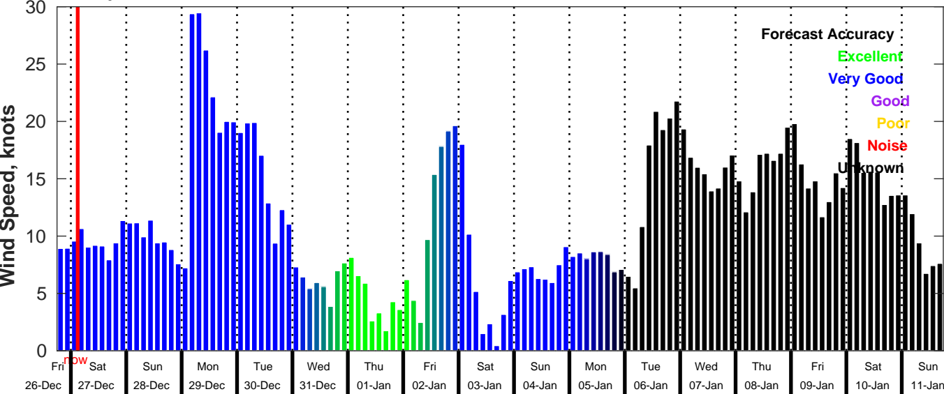
GFS Wind Speed Forecast for NDBC 42035 from 26-Dec-2025 18:00:00 to 11-Jan-2026 18:00:00
