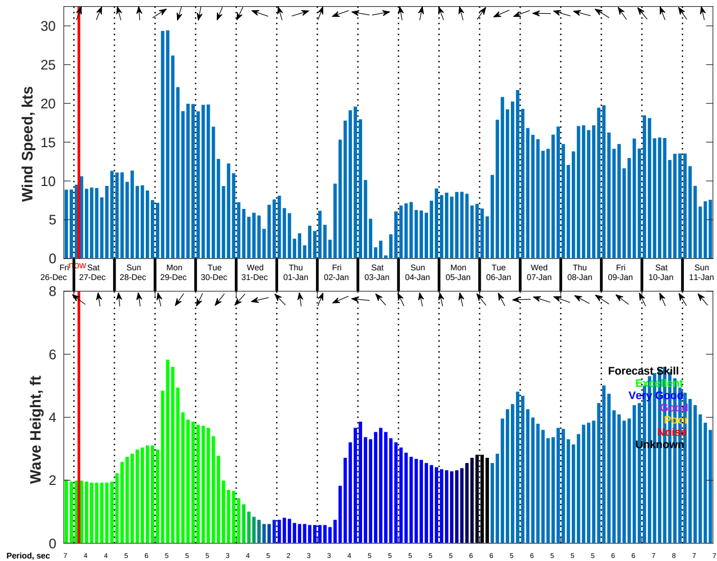
Wind & Wave Forecast for NDBC 42035 from 26-Dec-2025 18:00:00 to 11-Jan-2026 18:00:00
